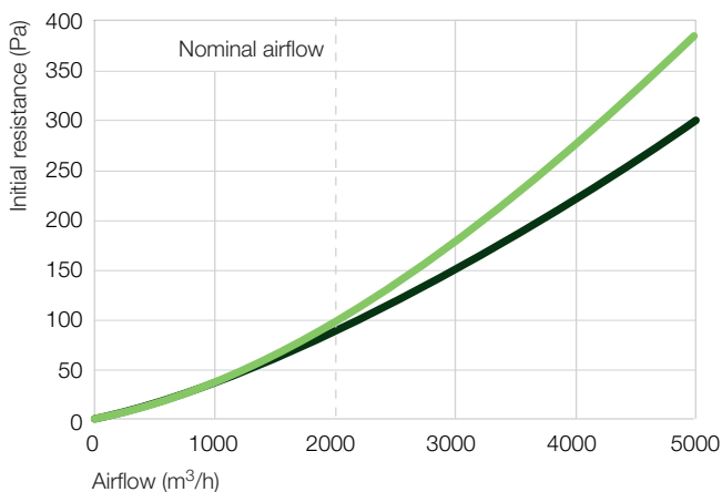
VariCel EcoPak - ePM1 55% 592x592x48 / ePM10 70% 592x592x48
