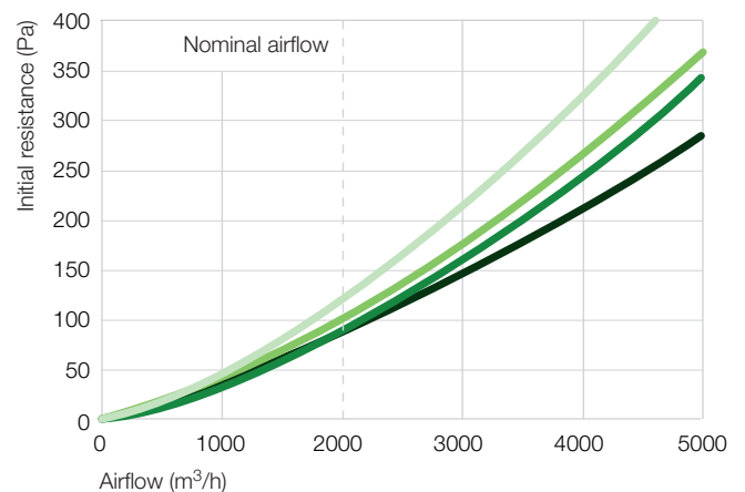
VariPak - ePM1 80% 592x592x98 / ePM1 65% 592x592x98 / ePM1 55% 592x592x98 / ePM10 592x592x98
