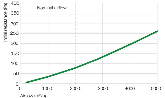
VariCel EcoPak - ePM1 55% 592x592x98
