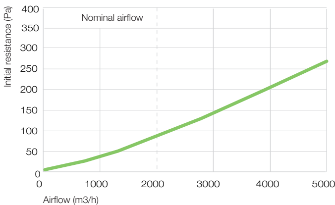
VariCel EcoPak - ePM1 55% 592x592x48
